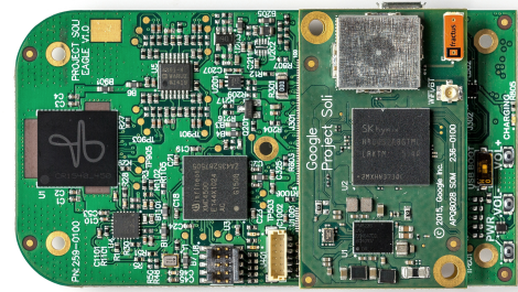
Figure 10: The Soli chip is easily integrated into development boards as shown here, as well as consumer devices.
